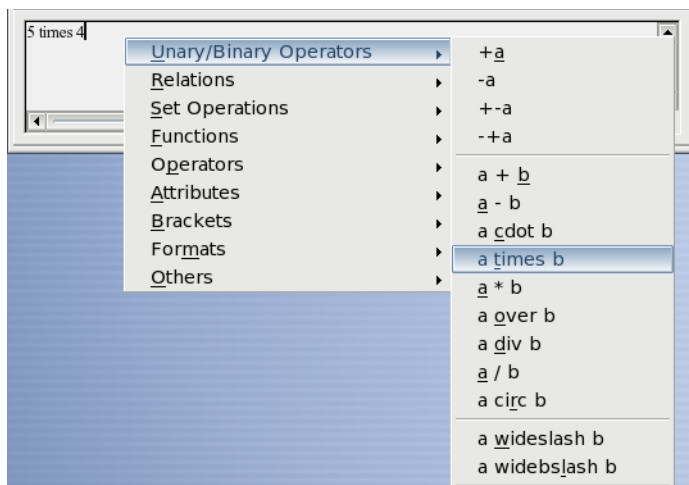
Figure 6. Right-click menu
